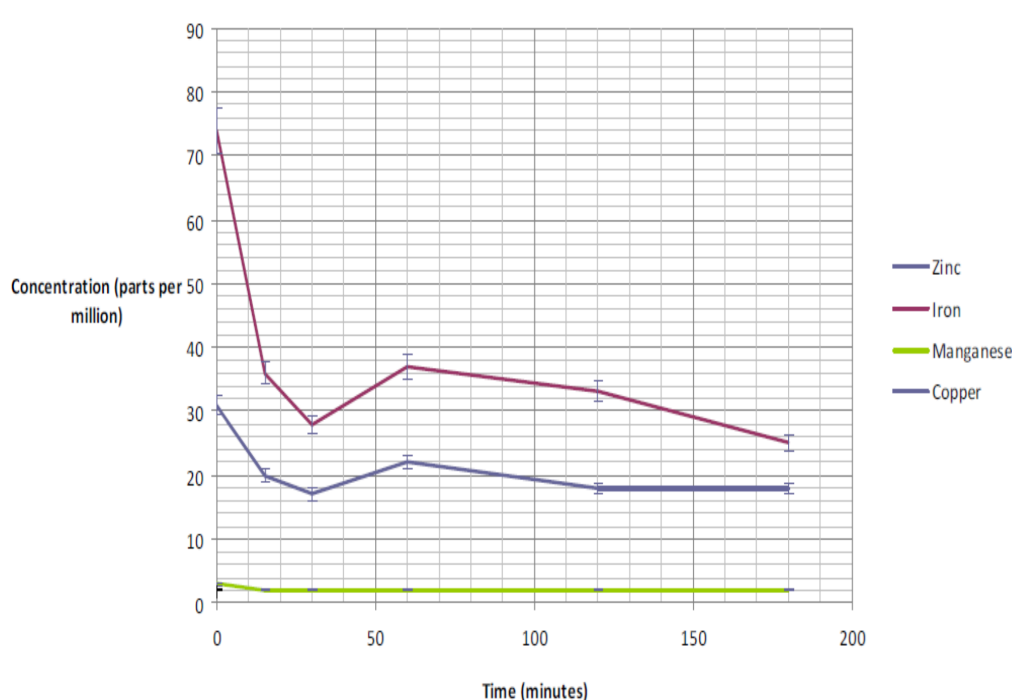
The Removal of Heavy Metal Ions from Wheal Jane Water by Zeolite (8g) Absorption
