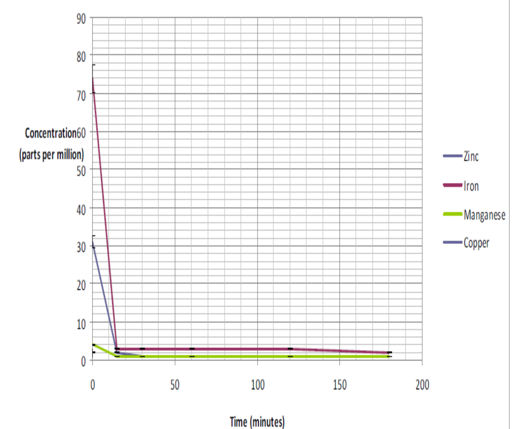
The Removal of Metal Ions from Wheal Jane Water by Material X
